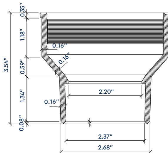
SIDE CUT VIEW
