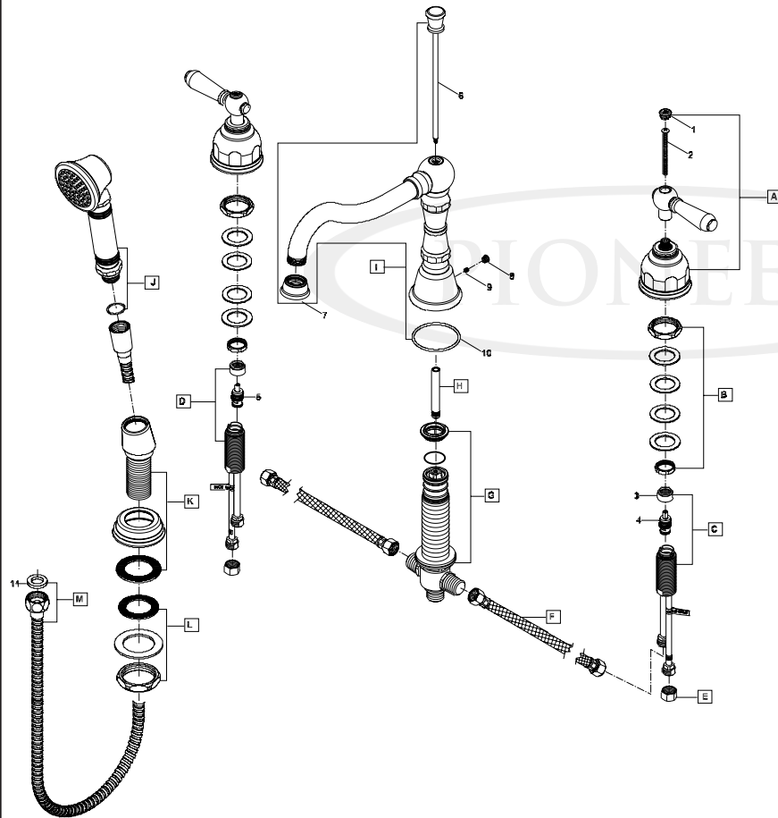
Product Diagram
