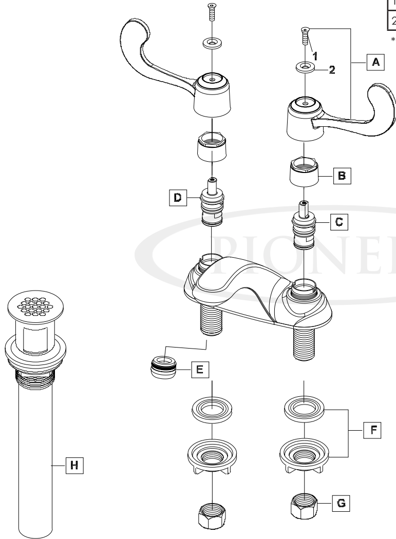
Product Diagram
