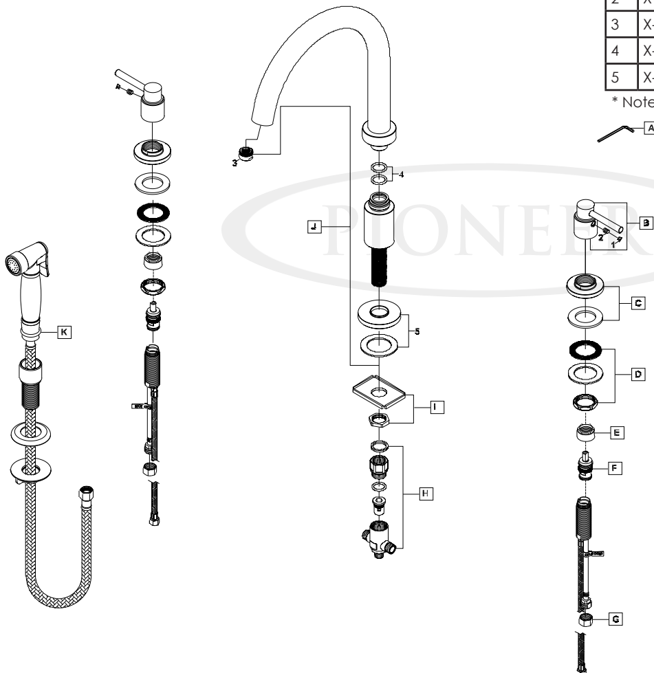
Product Diagram
