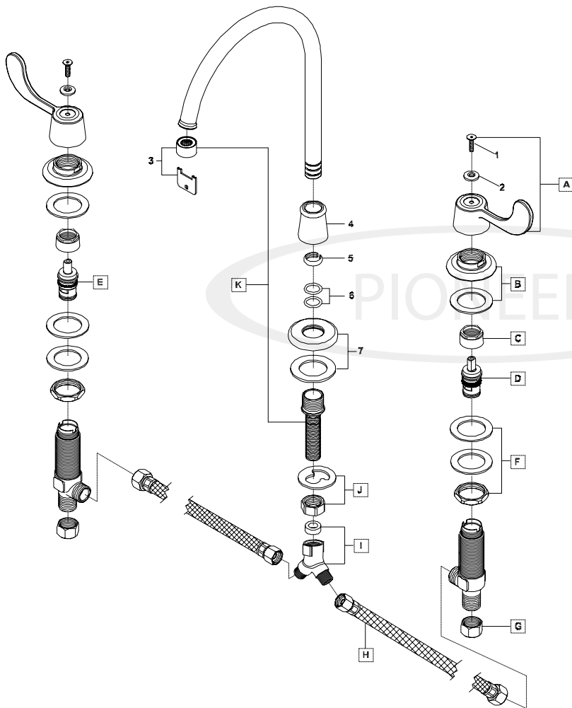
Product Diagram
