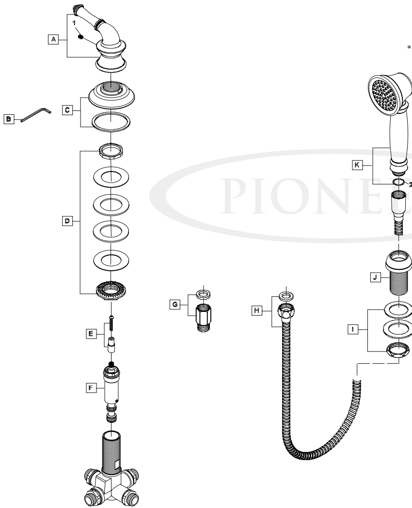
Product Diagram
