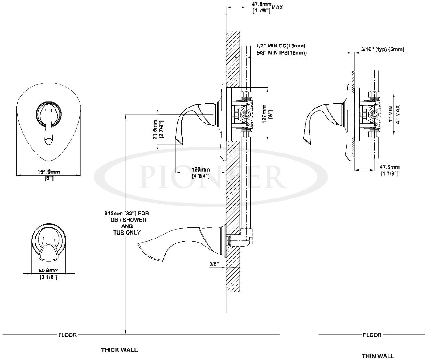
Product Diagram
