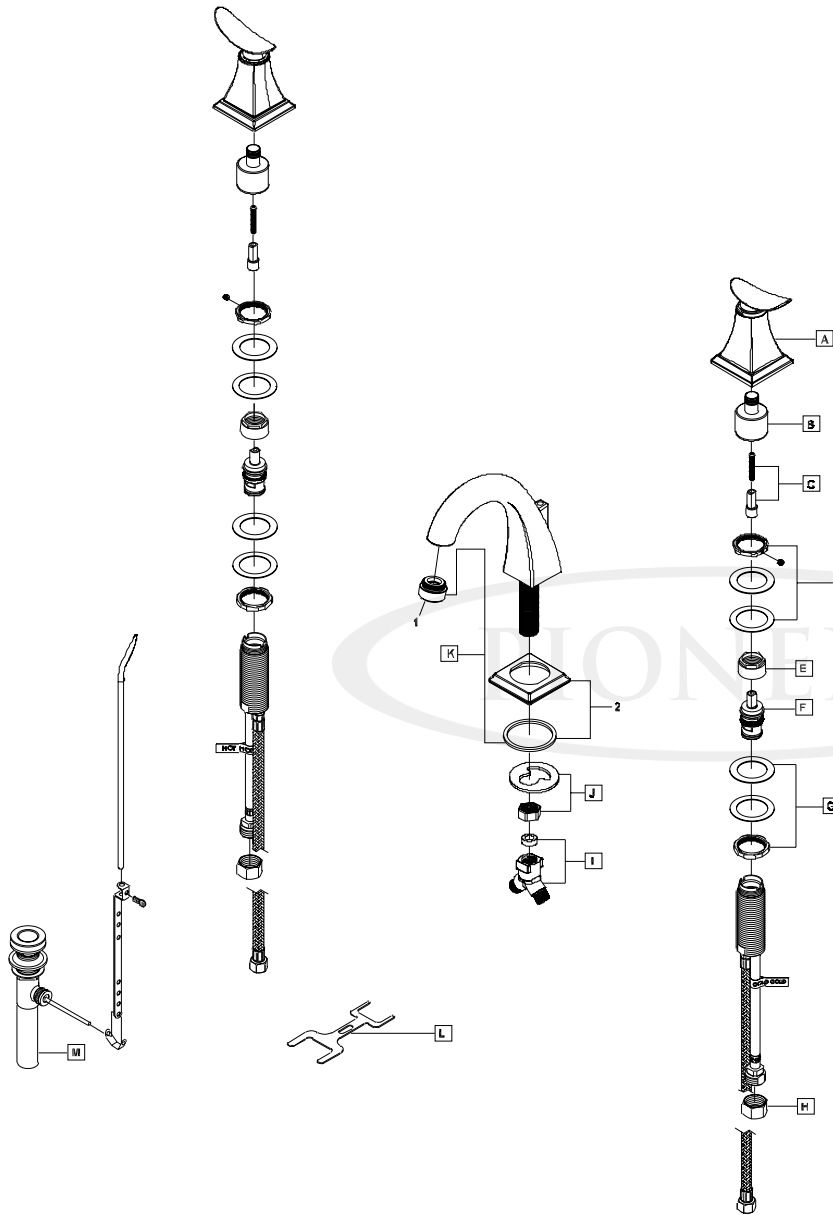
Product Diagram
