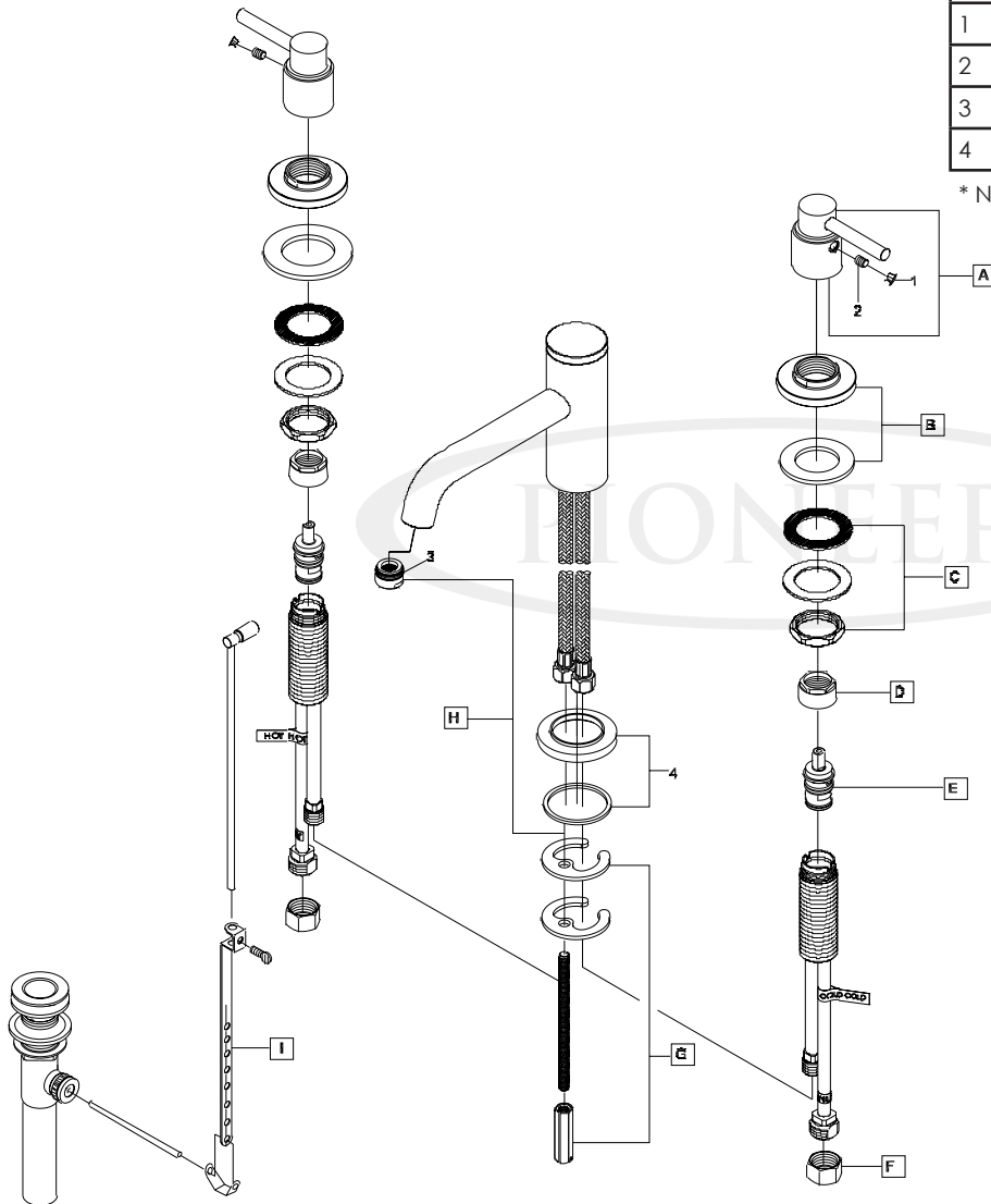
Product Diagram
