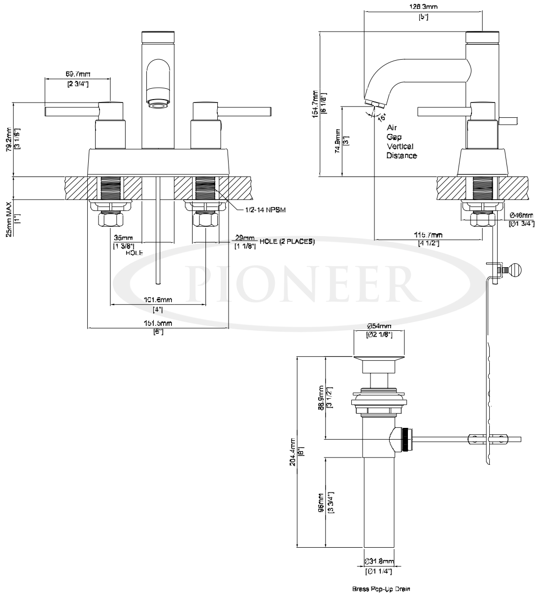
Product Diagram
