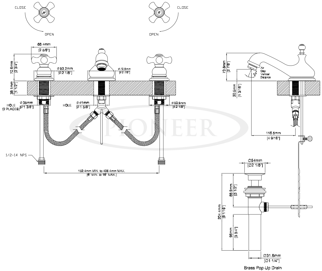
Product Diagram
