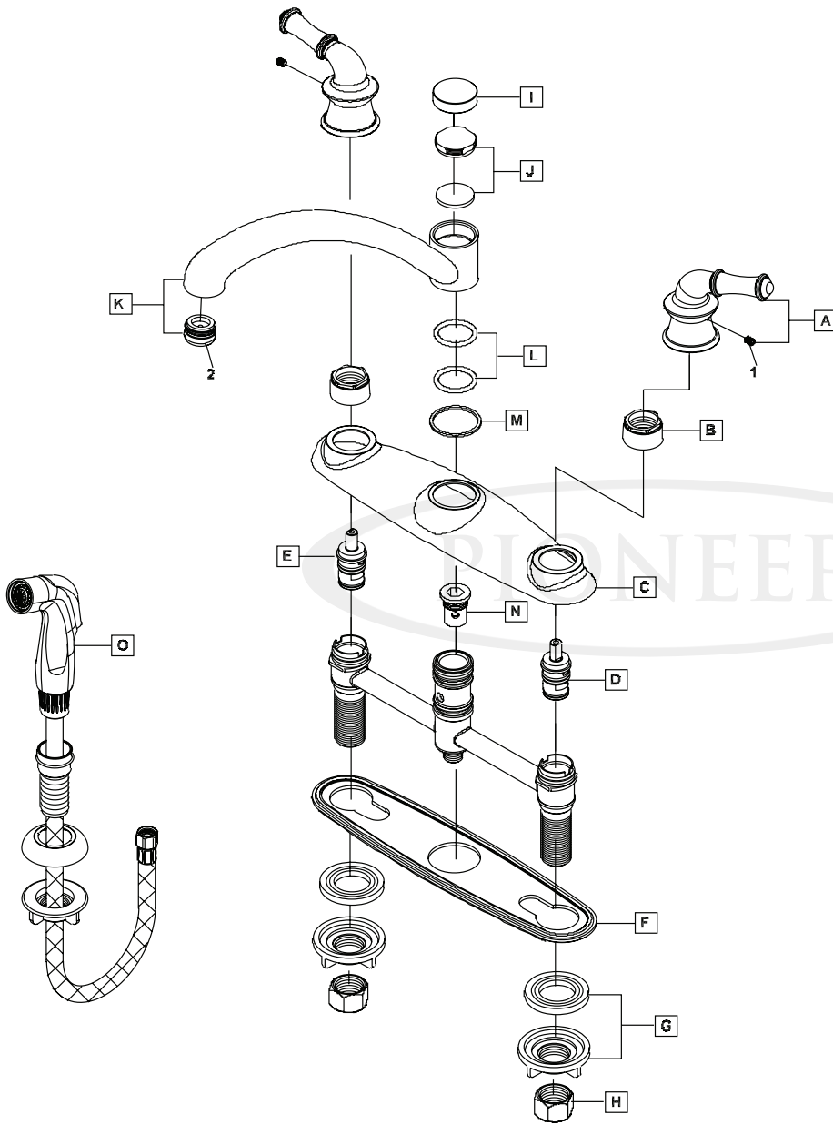
Product Diagram
