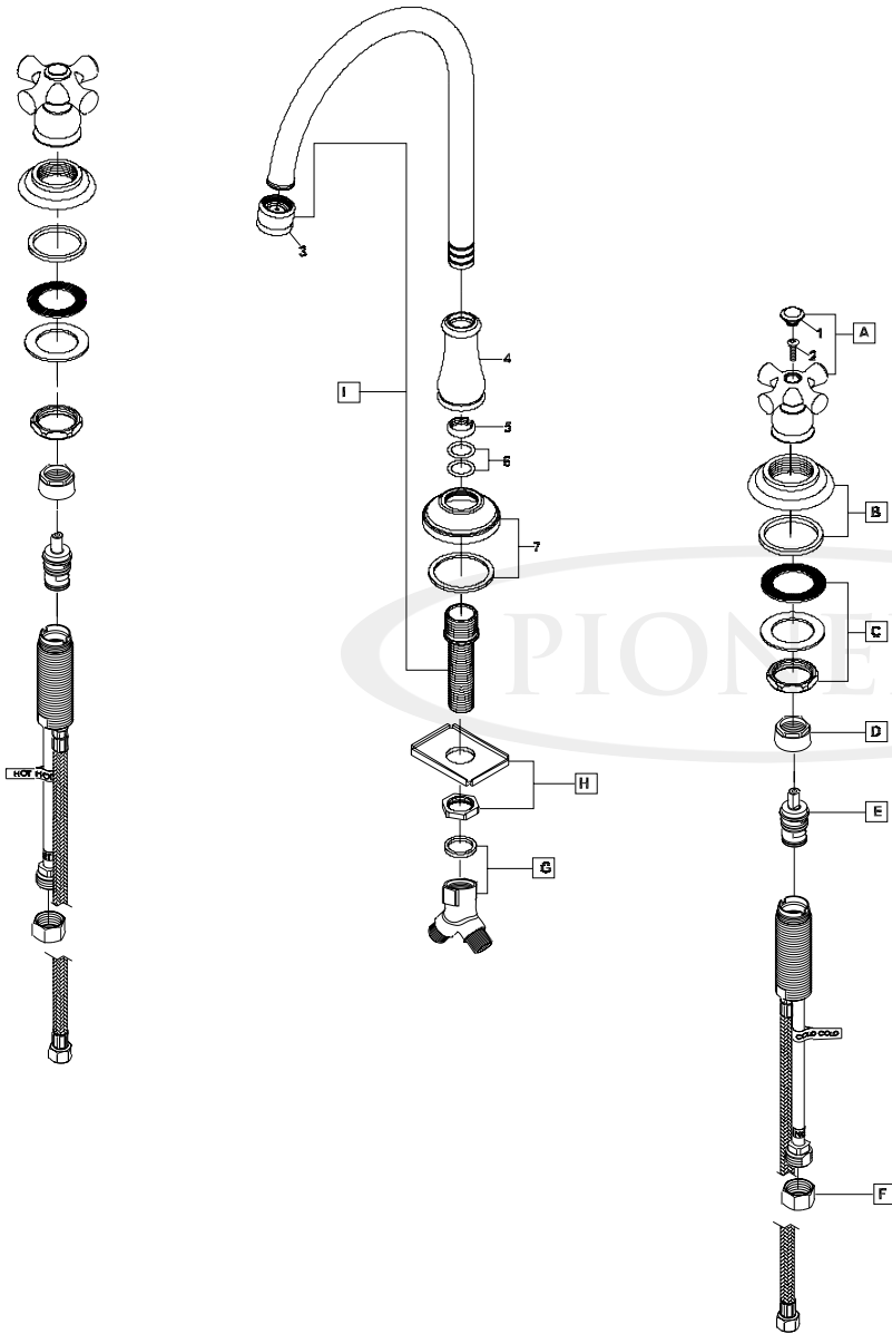
Product Diagram
