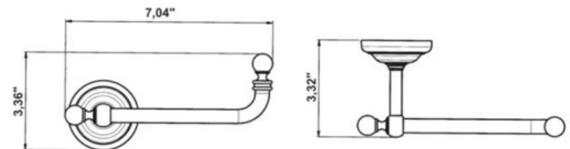
paper roll holder
