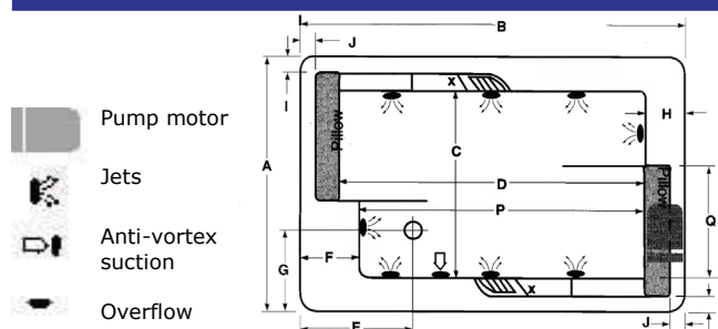
Tub must be set in Mortar Base
