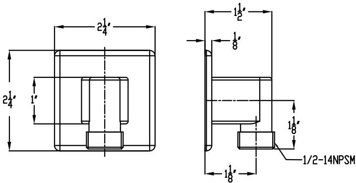
Supply Elbow
