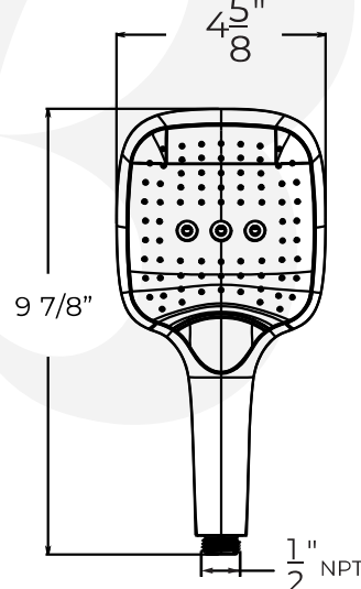
Hand Shower
