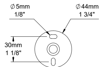
Plaque de montage Mounting plate
