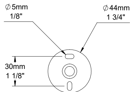
Plaque de montage Mounting plate
