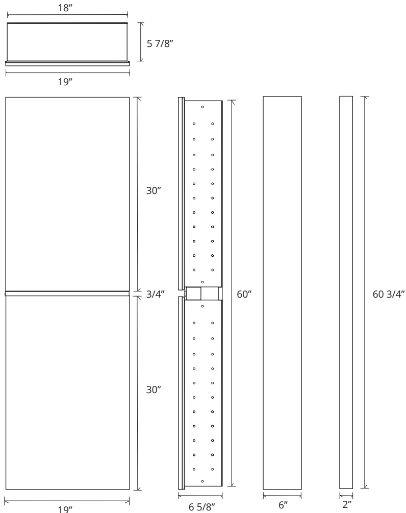
Side Mirror Kit SMK6-60 Order for Surface Mount Side Mirror Kit SRMK2-60 Order for Semi-Recessed Mount
