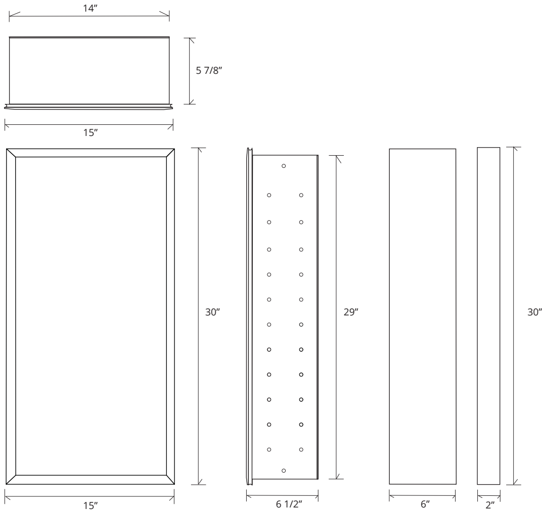
Beveled Mirror Section View
