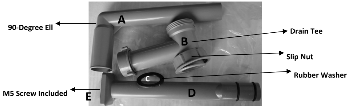
Drain Parts supplied by Dawn (can be used to replace items in the dotted area above)
